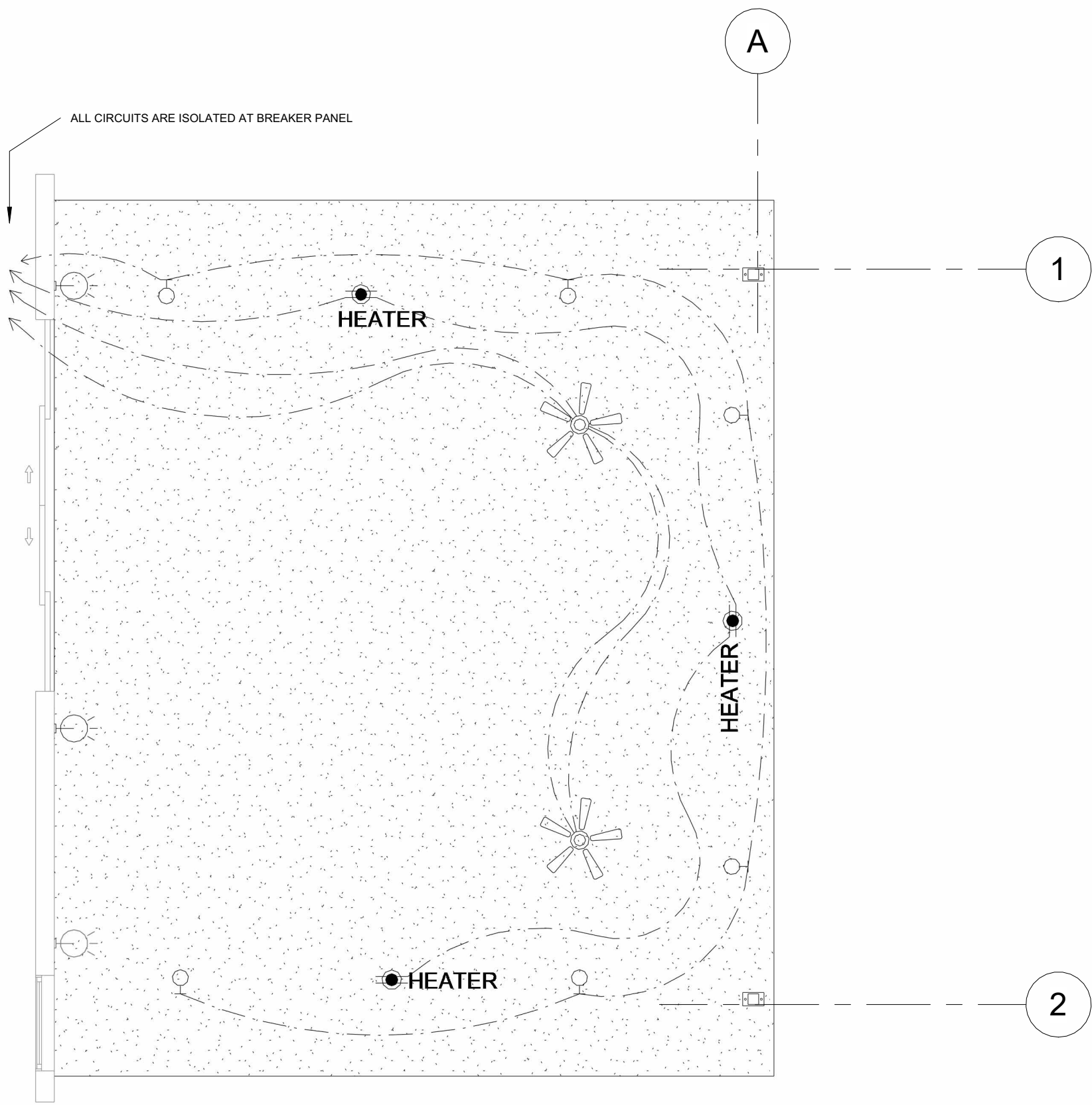
1 ELECTRICAL PLAN 1/4" = 1'-0"
